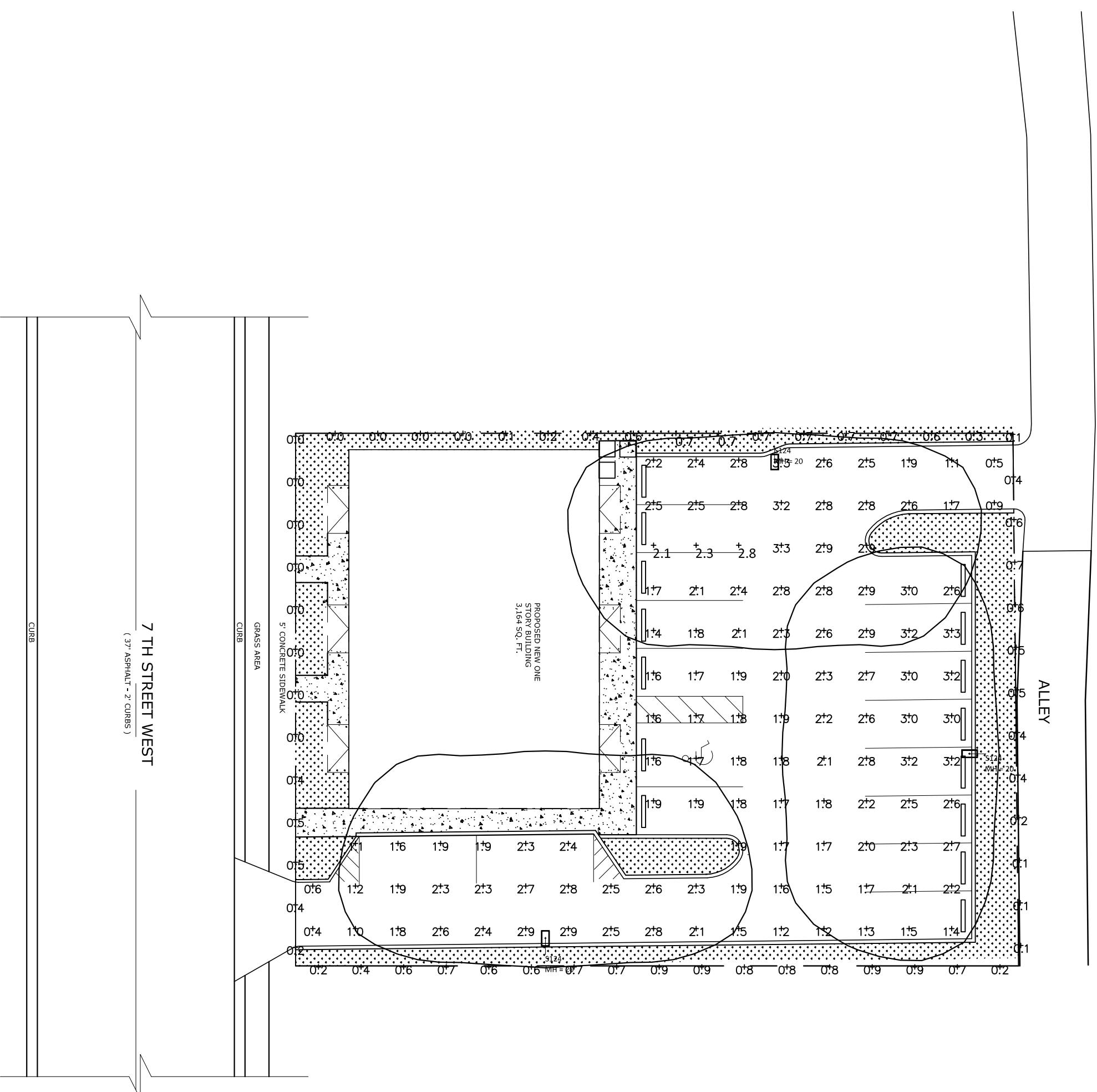
SITE LIGHTING PLAN SCALE : 1" = 20'-0"
