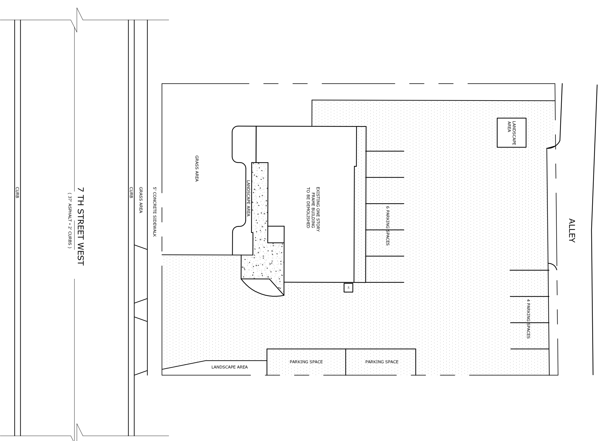
EXISTING SITE PLAN SCALE : 1" = 20'-0"
